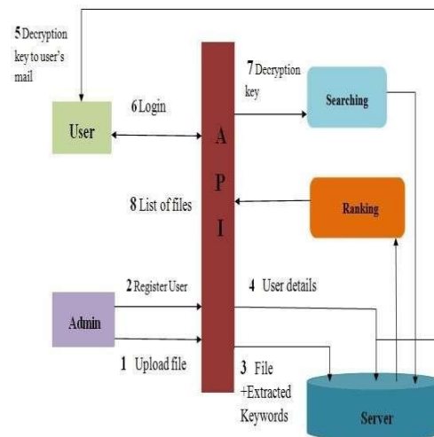
Figure 3: System architecture
